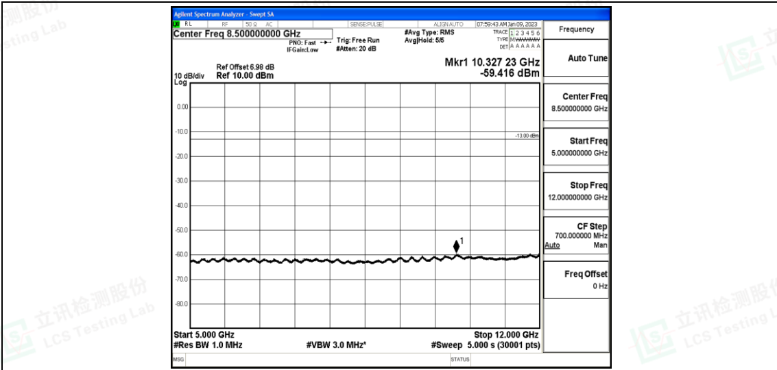
Band12-10MHz-16QAM-23095-1-0-Low-5000-12000--59.42-PASS
