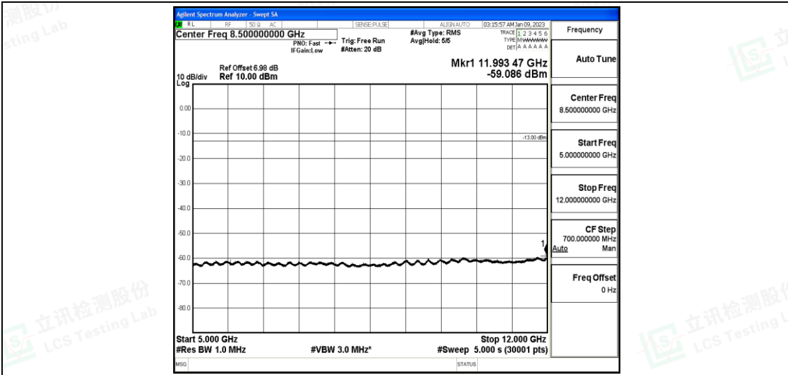
Band12-3MHz-16QAM-23095-1-0-Low-5000-12000--59.09-PASS
