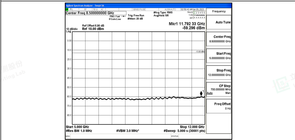
Band12-1.4MHz-16QAM-23095-1-0-Low-5000-12000--59.3-PASS
