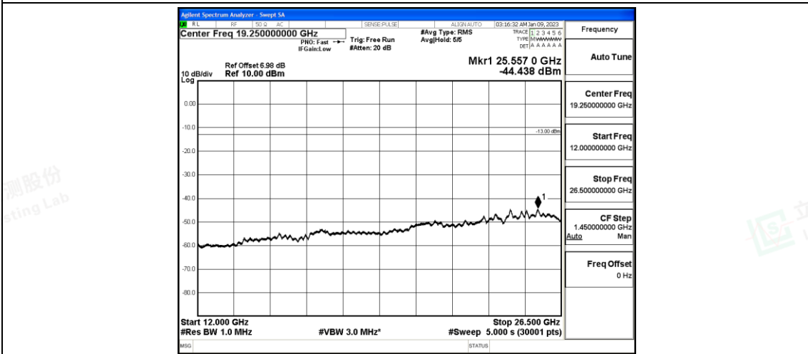
Band12-3MHz-16QAM-23095-1-0-Low-12000-26500--44.44-PASS
