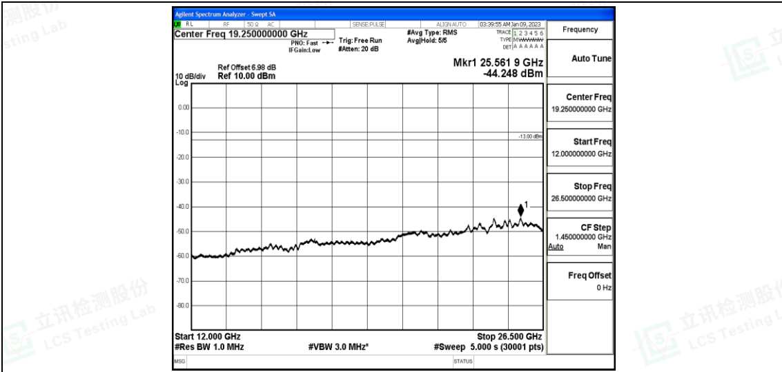
Band12-5MHz-QPSK-23095-1-0-Low-12000-26500--44.25-PASS
