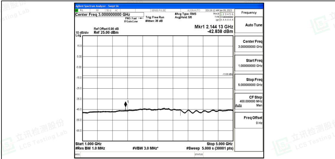
Band12-3MHz-16QAM-23165-1-0-High-1000-5000--42.84-PASS
