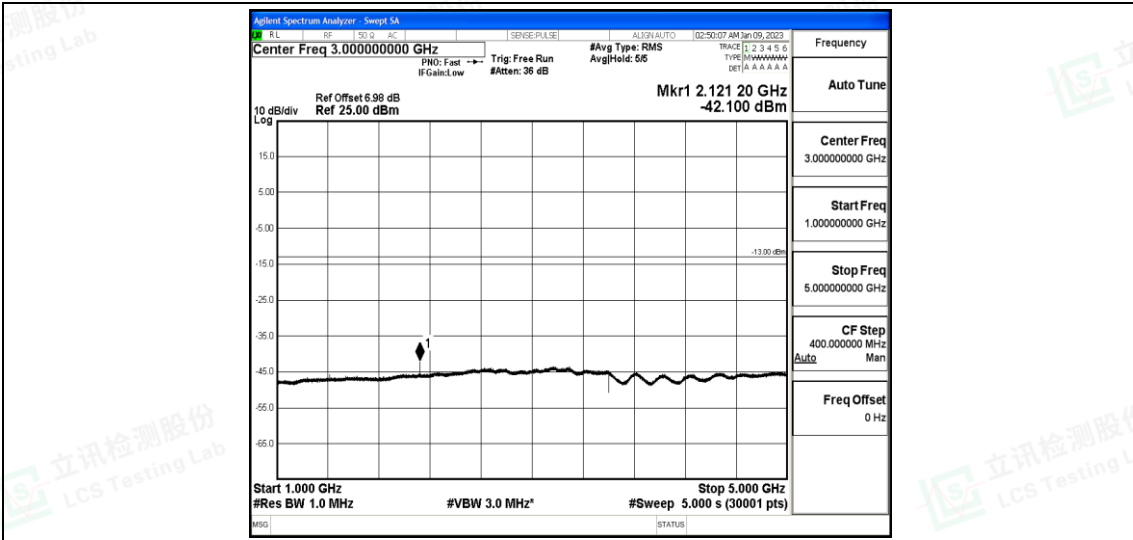
Band12-1.4MHz-16QAM-23095-1-0-Low-1000-5000--42.1-PASS
