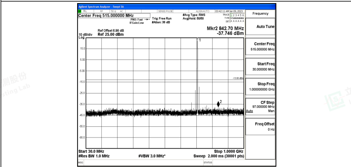
Band12-5MHz-QPSK-23155-1-0-High-30-1000--37.75-PASS
