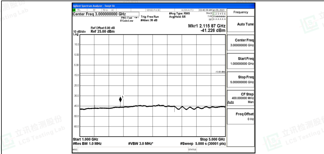
Band12-5MHz-16QAM-23095-1-0-Low-1000-5000--41.23-PASS
