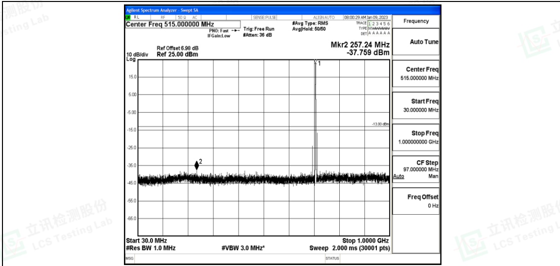
Band12-10MHz-QPSK-23130-1-0-High-30-1000--37.76-PASS
