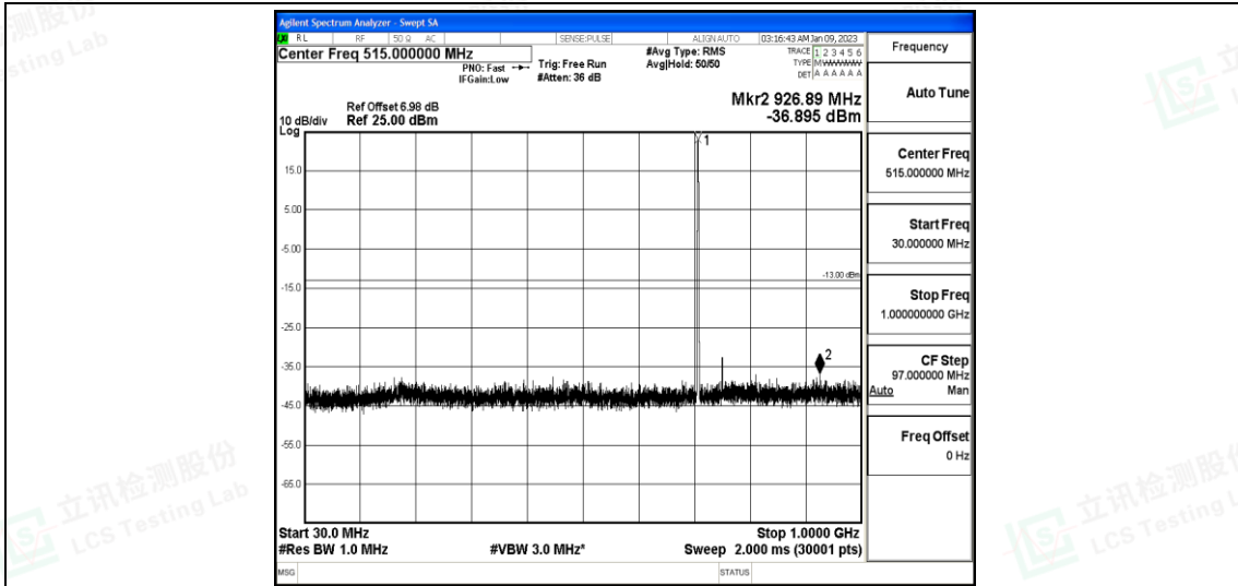
Band12-3MHz-QPSK-23165-1-0-High-30-1000--36.9-PASS
