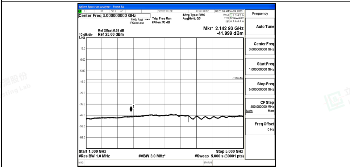
Band12-10MHz-QPSK-23130-1-0-High-1000-5000--42-PASS
