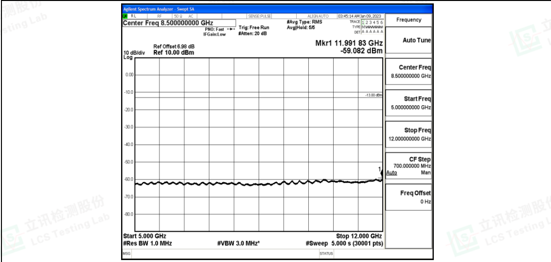
Band12-5MHz-16QAM-23155-1-0-High-5000-12000--59.08-PASS
