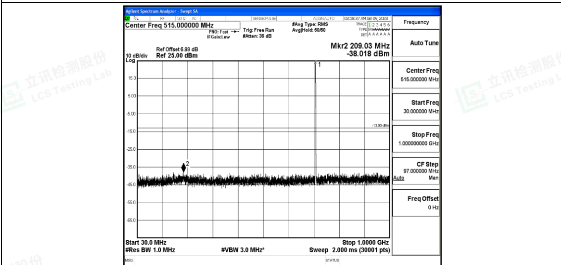
Band12-3MHz-16QAM-23165-1-0-High-30-1000--38.02-PASS
