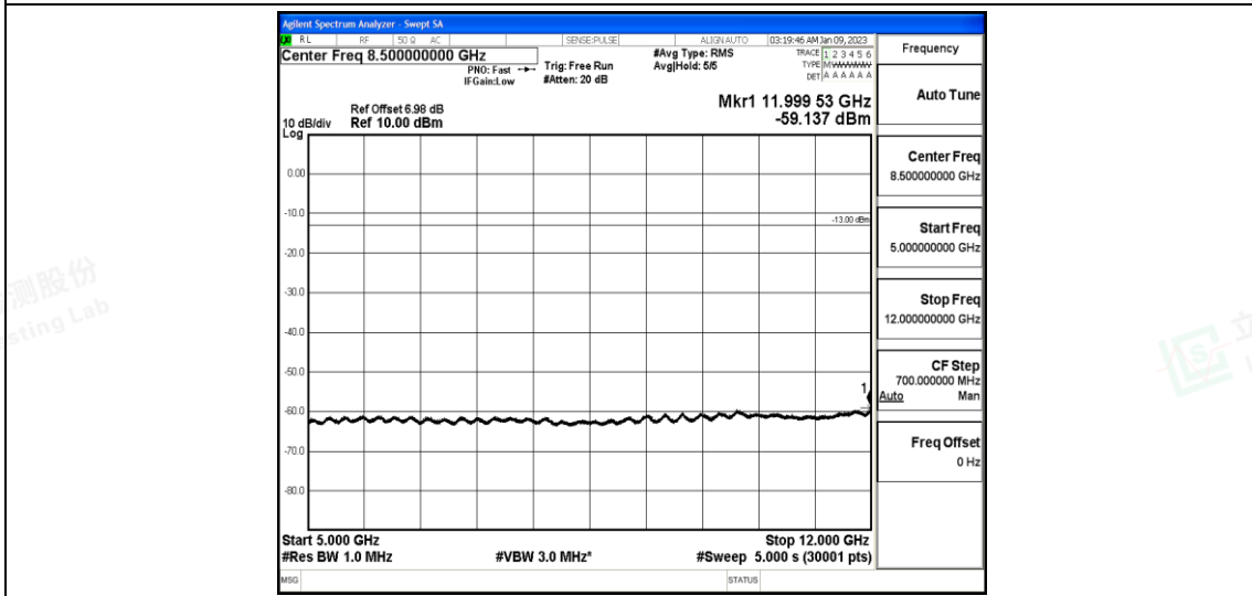
Band12-3MHz-16QAM-23165-1-0-High-5000-12000--59.14-PASS
