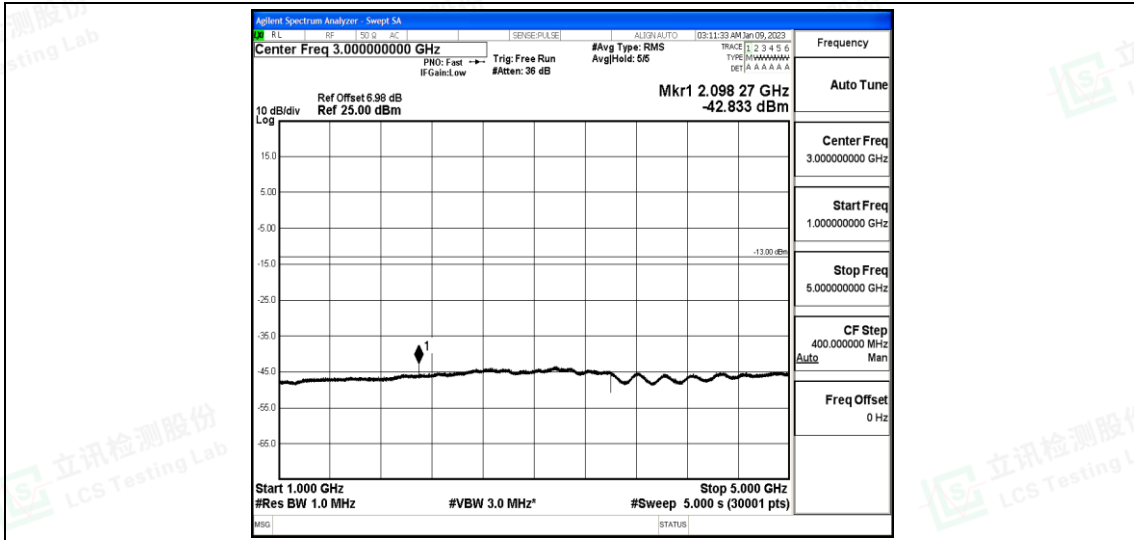
Band12-3MHz-16QAM-23025-1-0-Low-1000-5000--42.83-PASS
