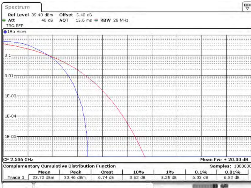
Band41-20MHz-QPSK-39750-100RB#0
