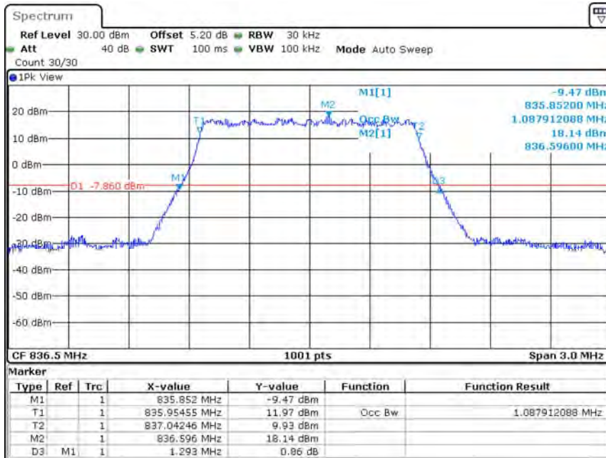
Band26-1.4MHz-QPSK-26915-6RB#0-1.088
