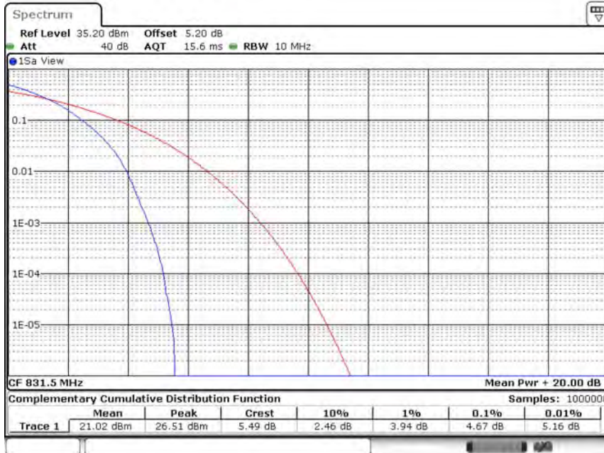
Band26-15MHz-QPSK-26865-75RB#0
