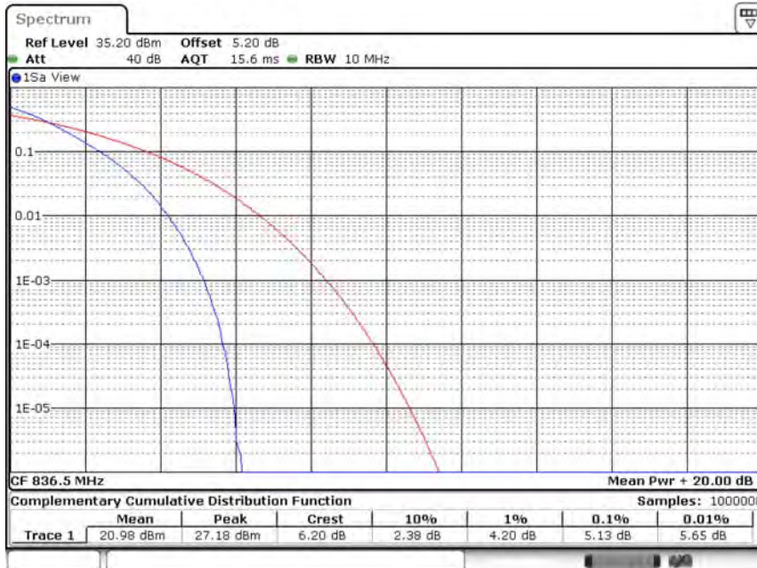
Band26-15MHz-QPSK-26915-75RB#0
