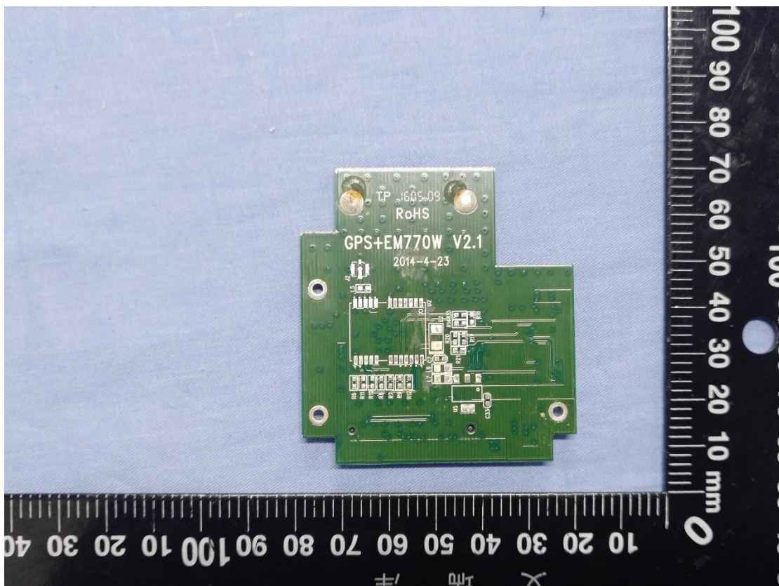
6. sub board bottom view
