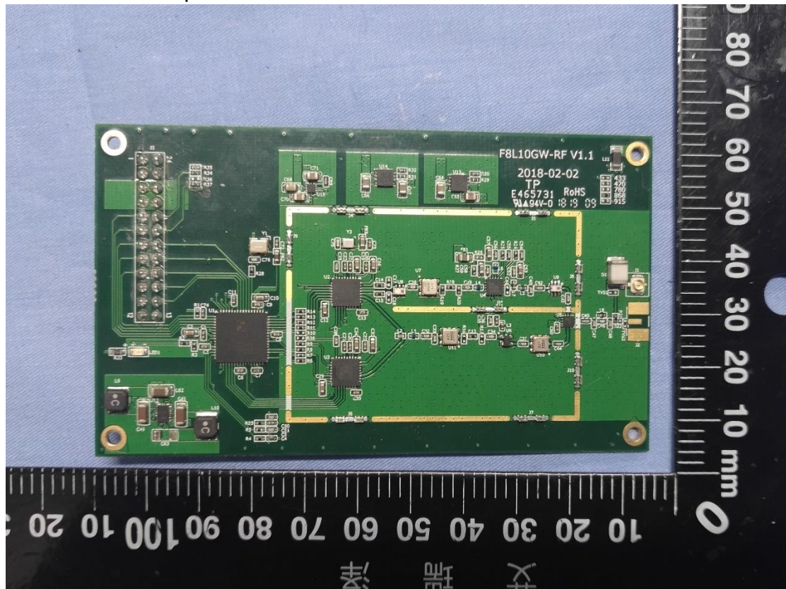
10.LoRa module bottom view
