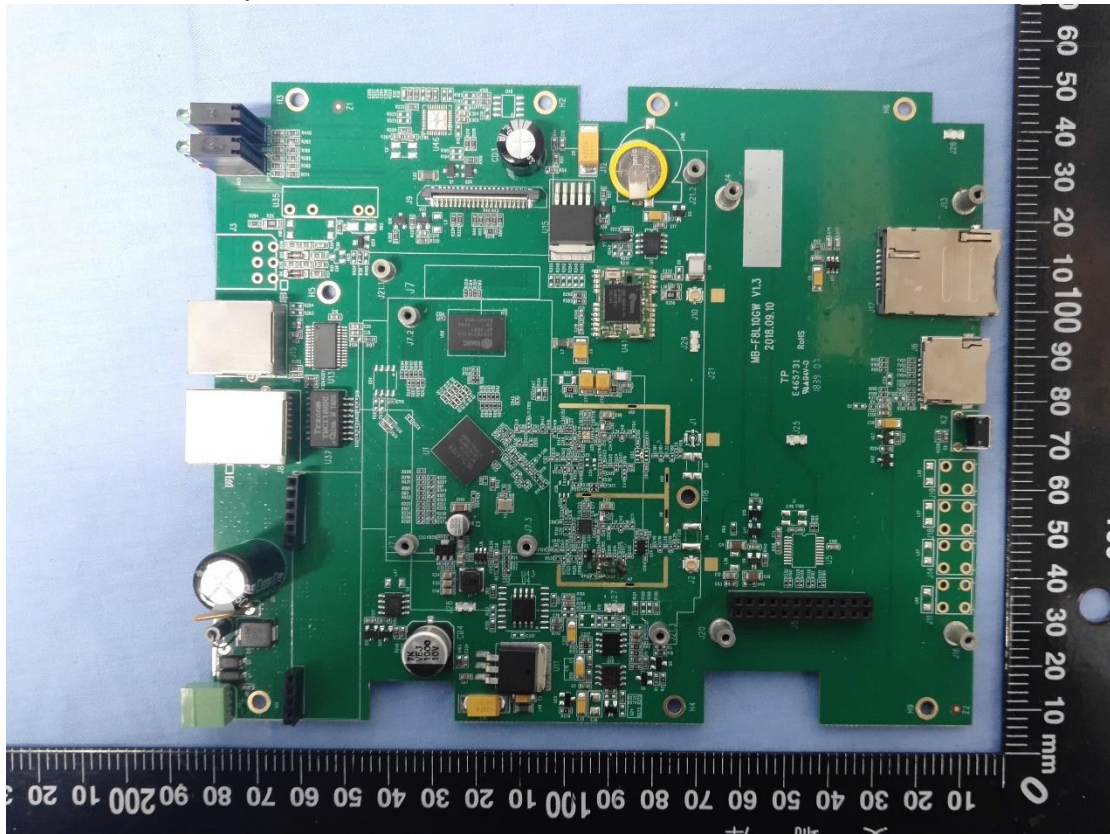
12.main board bottom view
