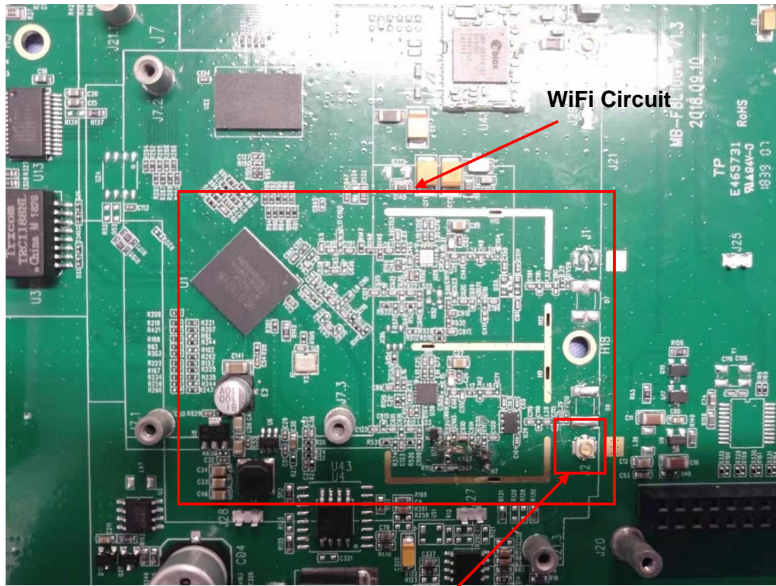
WiFi antenna connector
