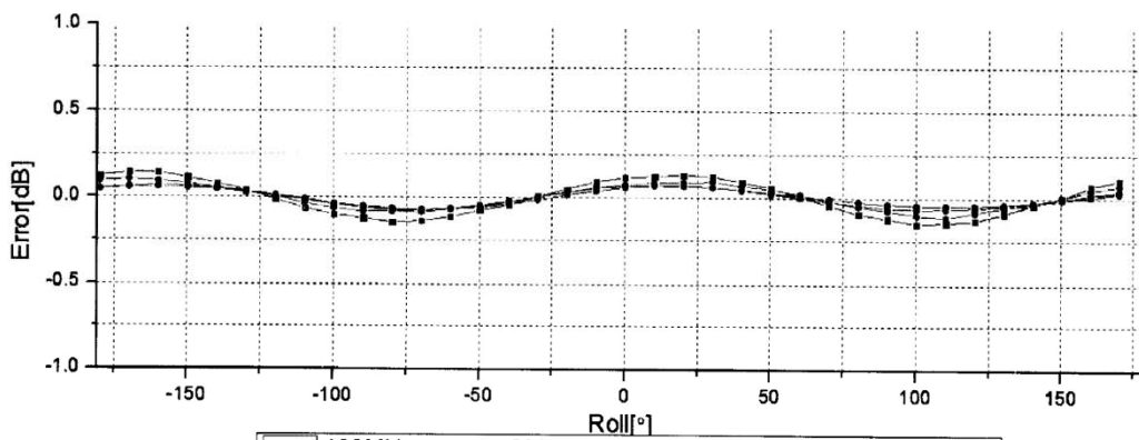
Uncertainty of Axial Isotropy Assessment: \pm 1.2\% (k=2)
