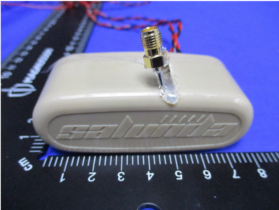
Conducted sample with temporary ZigBee antenna port
