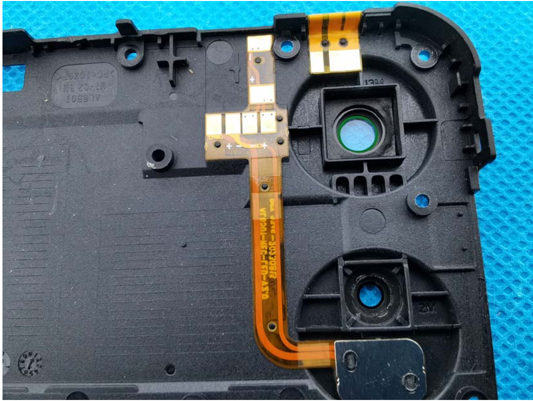
WIFI/BT/BLE/GPS Antenna
