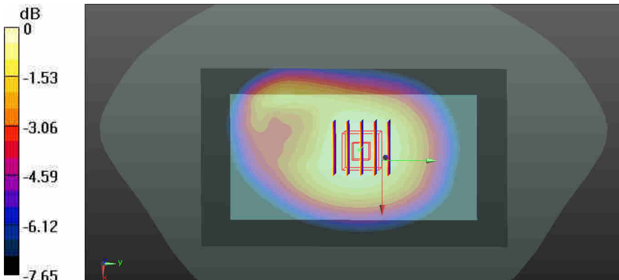
0 dB = 0.522 W/kg
