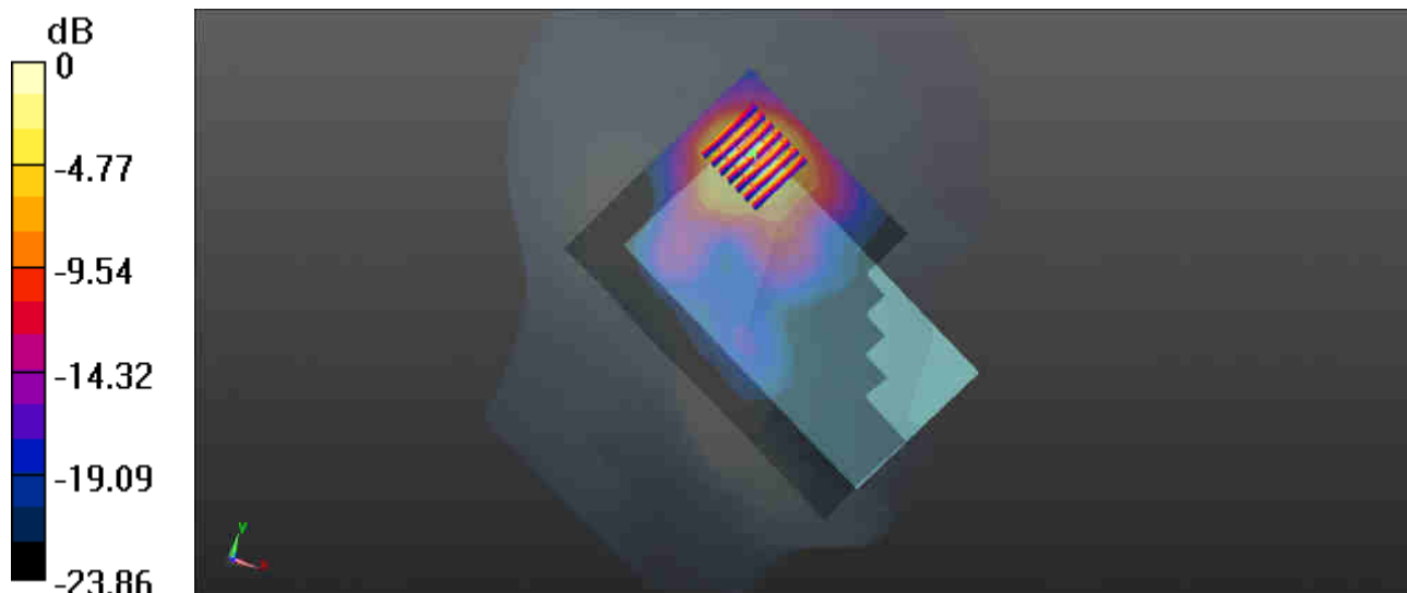
0 dB = 1.76 W/kg
