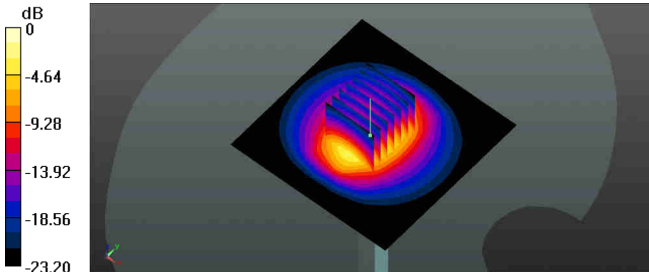
0 dB = 22.1 W/kg
