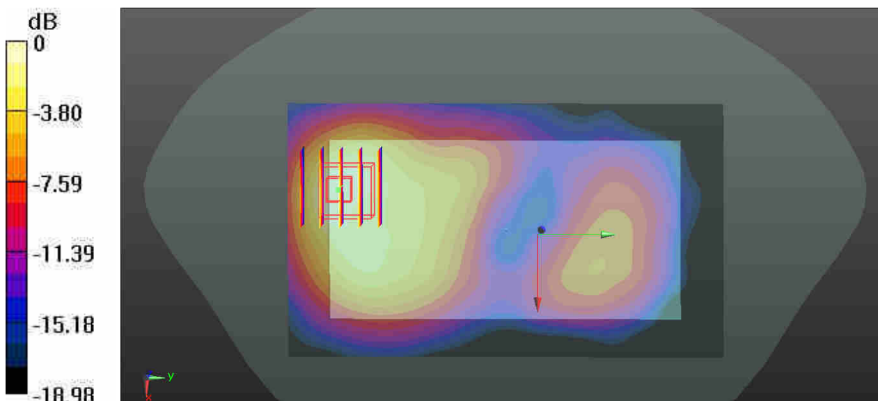
0 dB = 0.327 W/kg
