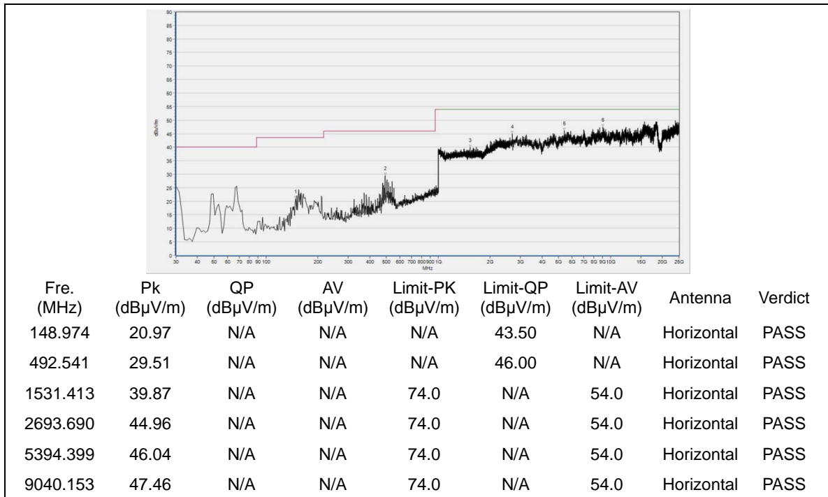
(30MHz to 25GHz, Antenna Horizontal @8-DPSK, channel 39)
