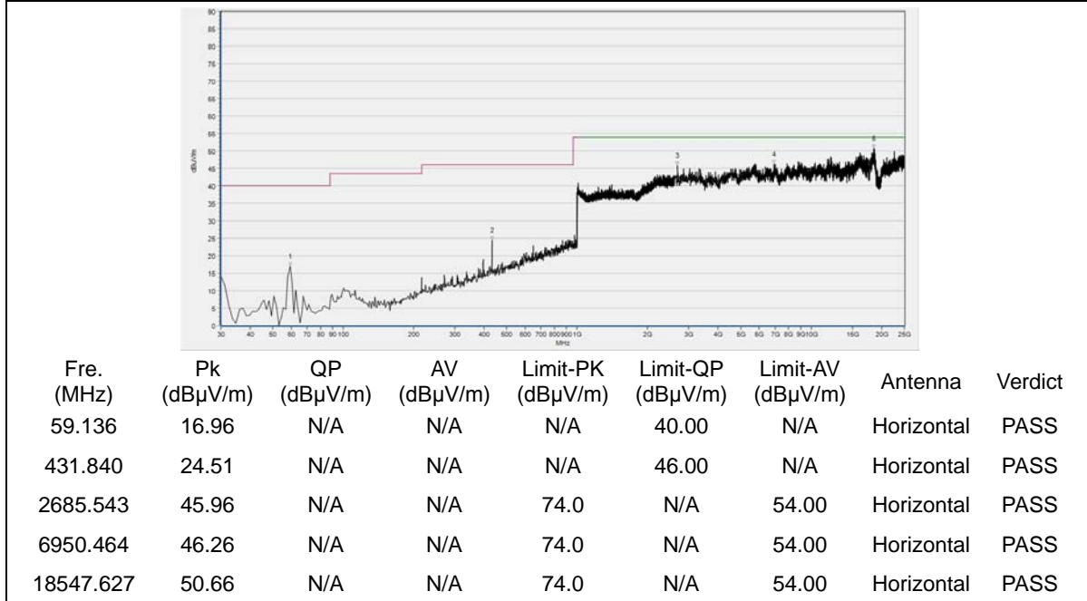
(30MHz to 25GHz, Antenna Horizontal @ \pi/4 -DQPSK, channel 0)
