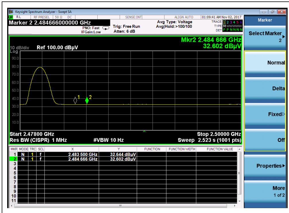
(Plot D2: Channel = 78 AVERAGE @ \pi/4 -DQPSK)
