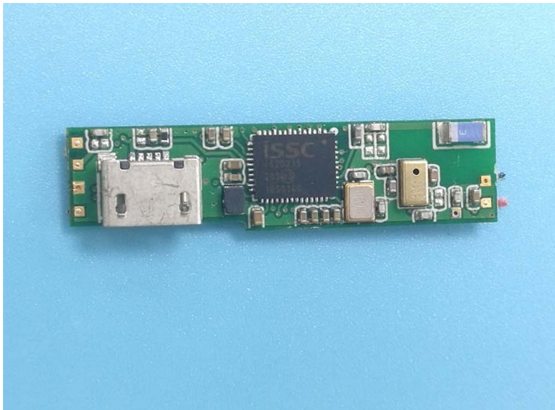
2. Mainboard front view
