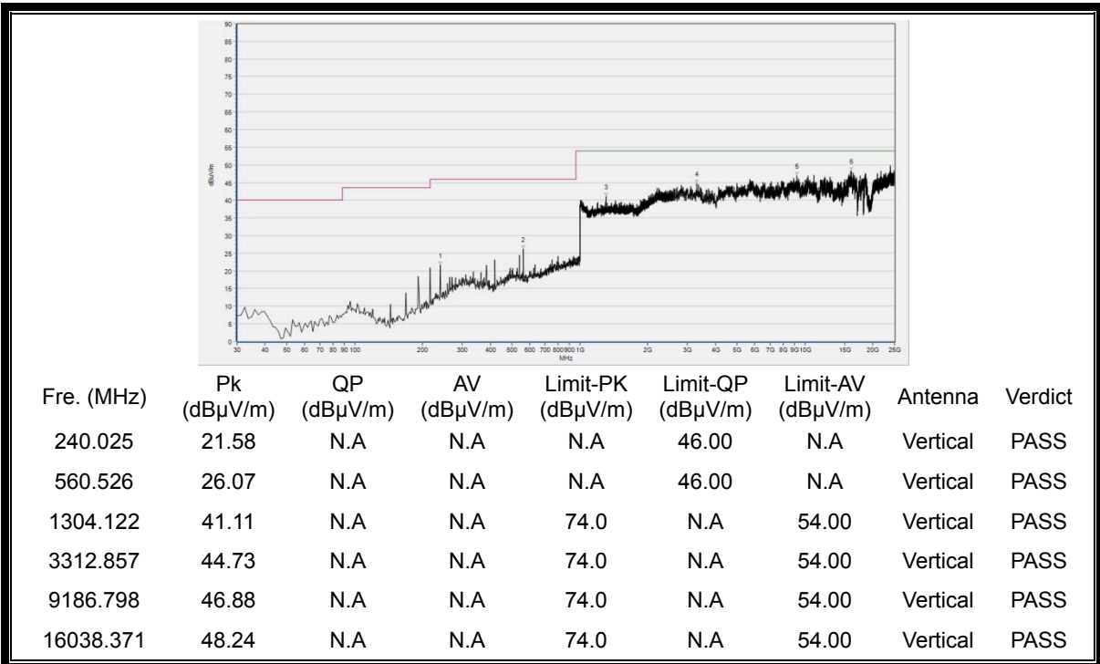
(30MHz to 25GHz, Antenna Vertical @ π/4-DQPSK, channel 78)
