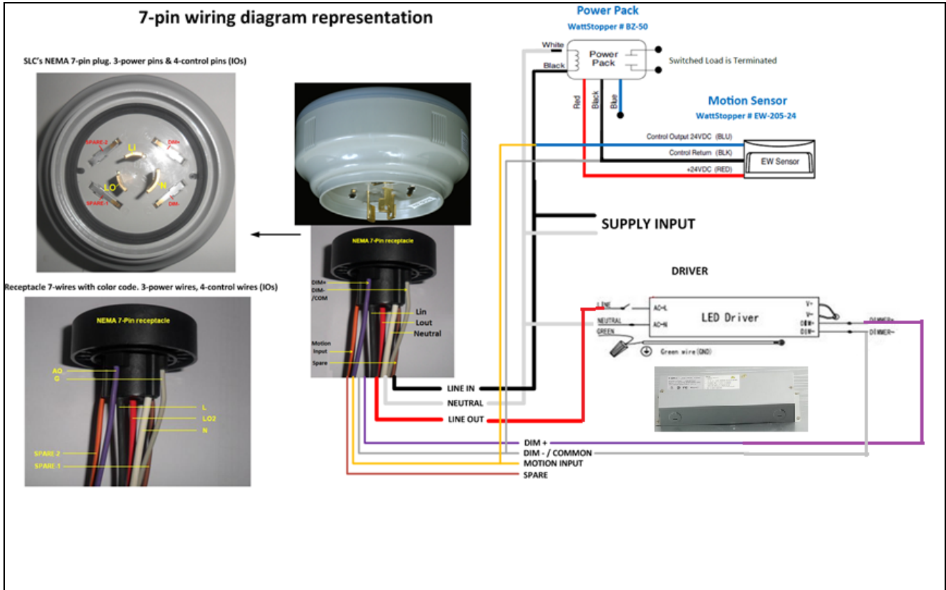
Fig. 2: Installation wiring diagram
