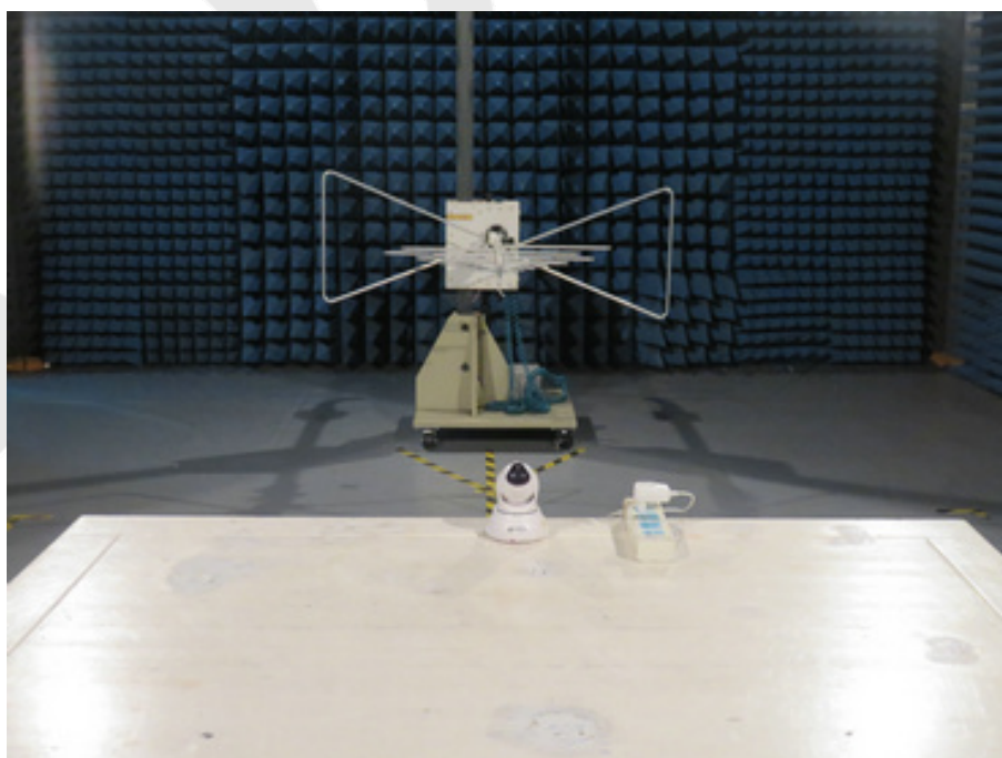
6.2. Photo of Radiation Emission Test
