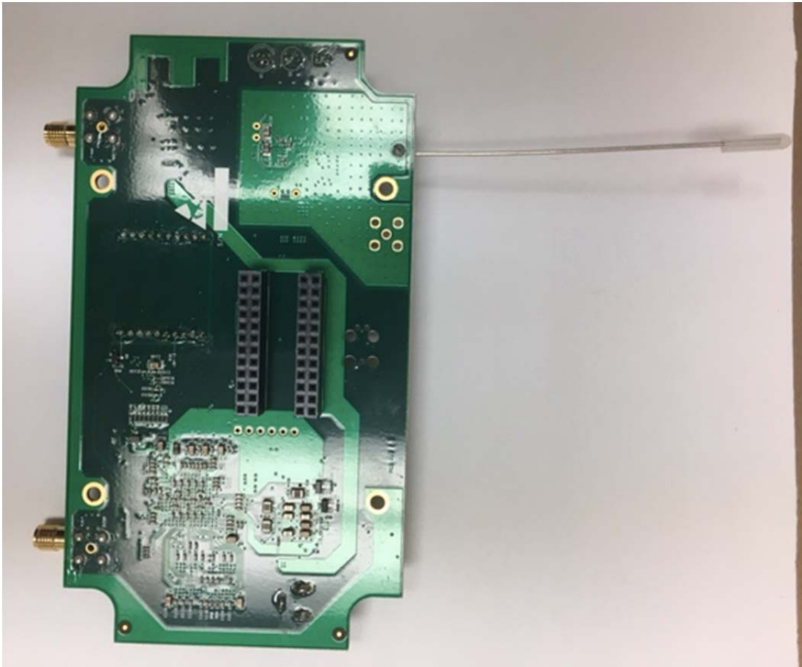
Bottom View
