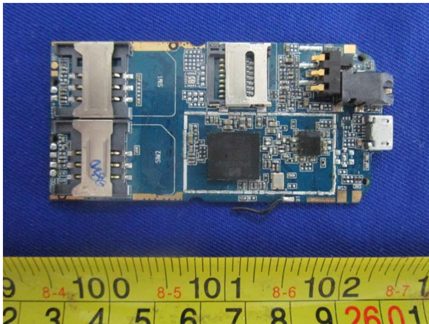
EUT – Board Top Uncover View
