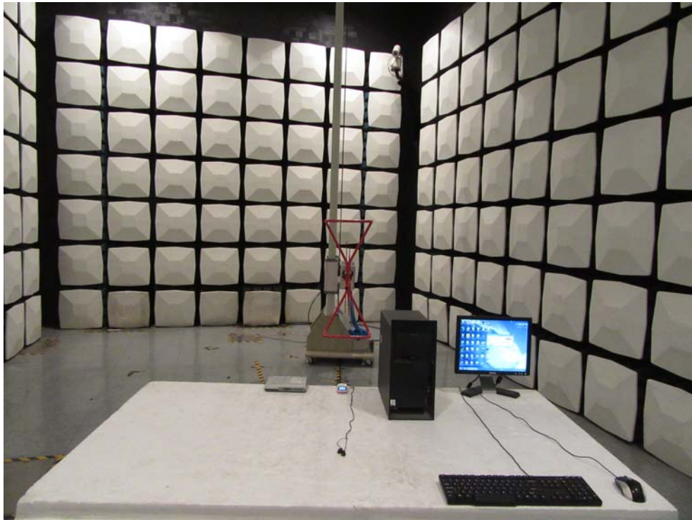
Radiated Emissions - Front View (Below 1GHz)
