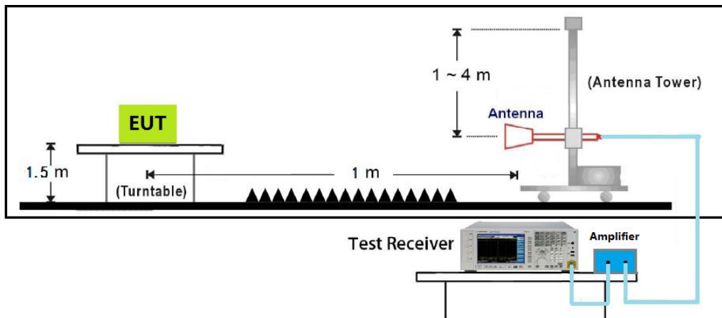
18GHz~40GHz Test Setup
