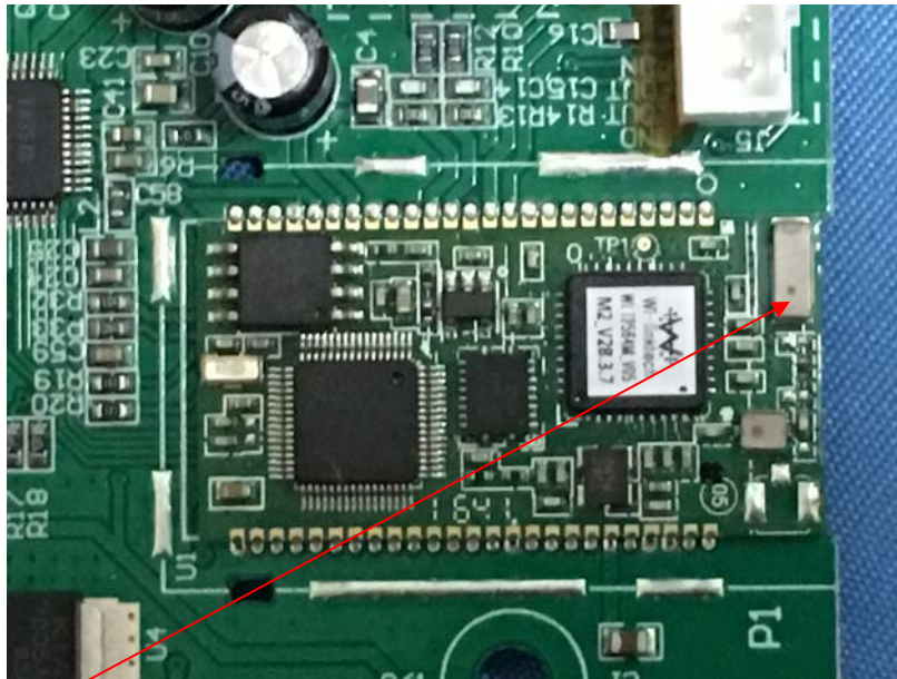
BT antenna(Chip Antenna)
