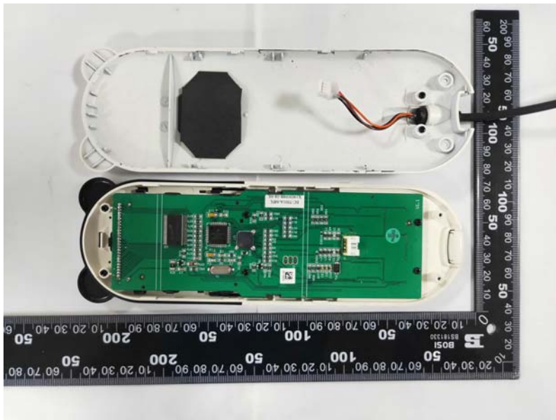
BT antenna(Chip Antenna)
