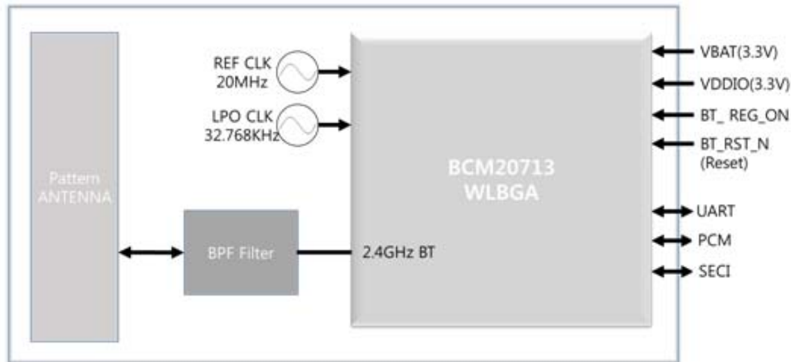
Figure.1 Block Diagram
