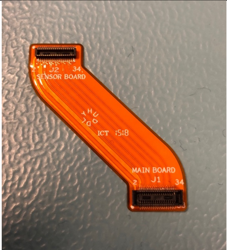
Bottom side of sensor FPC
