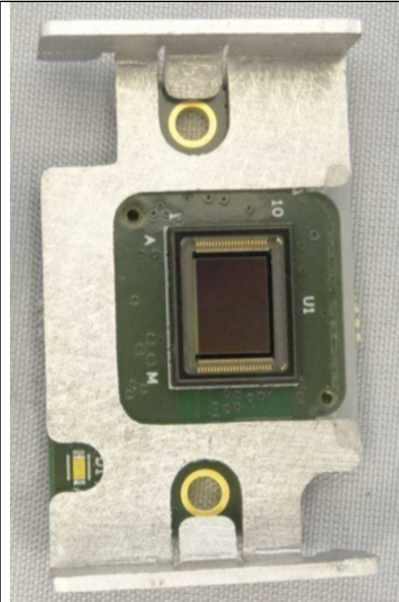
Top side of camera sensor PCB
