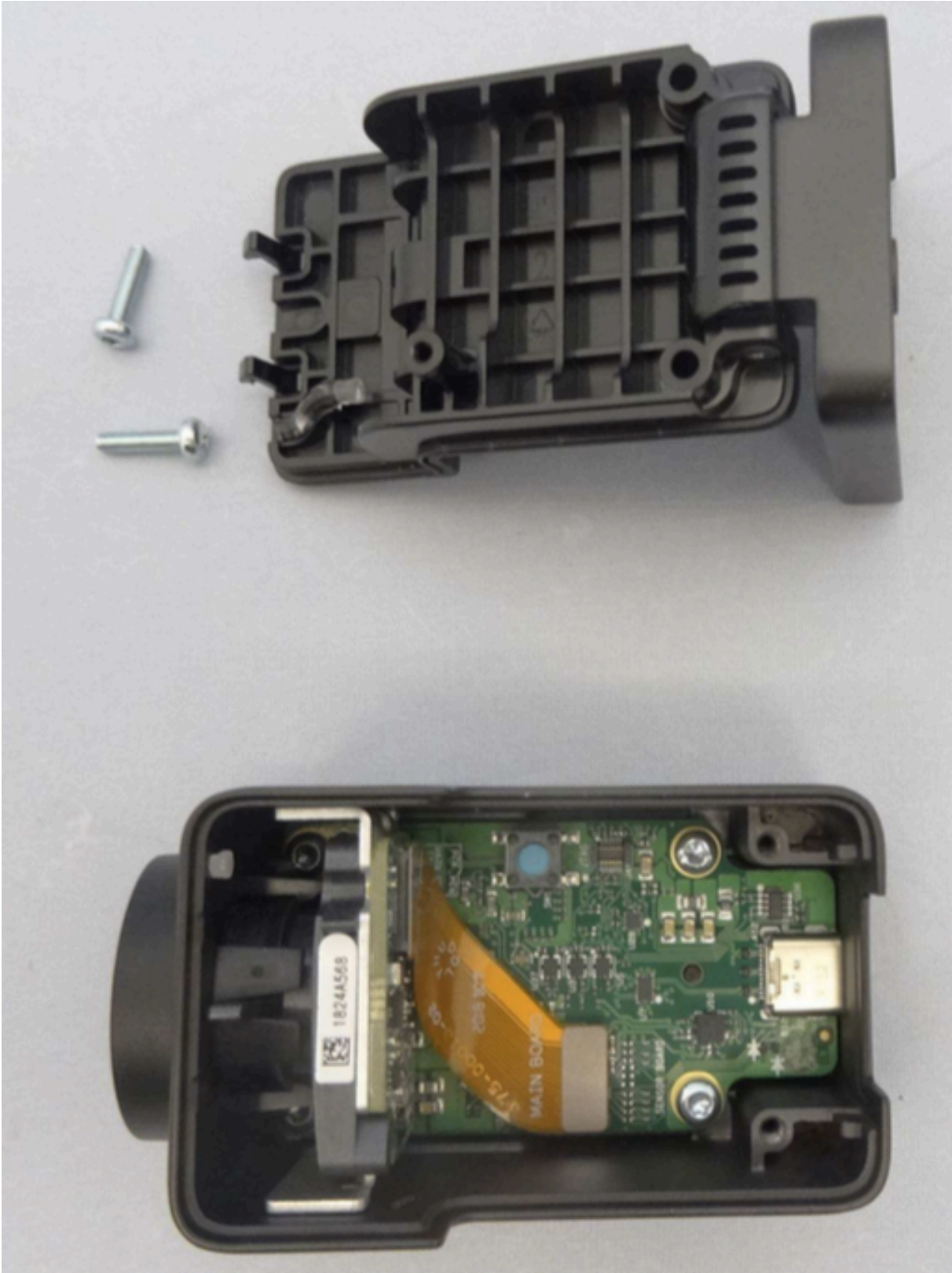
EUT, bottom side of enclosure disassembled. Mainboard PCB and camera sensor PCB can be seen
