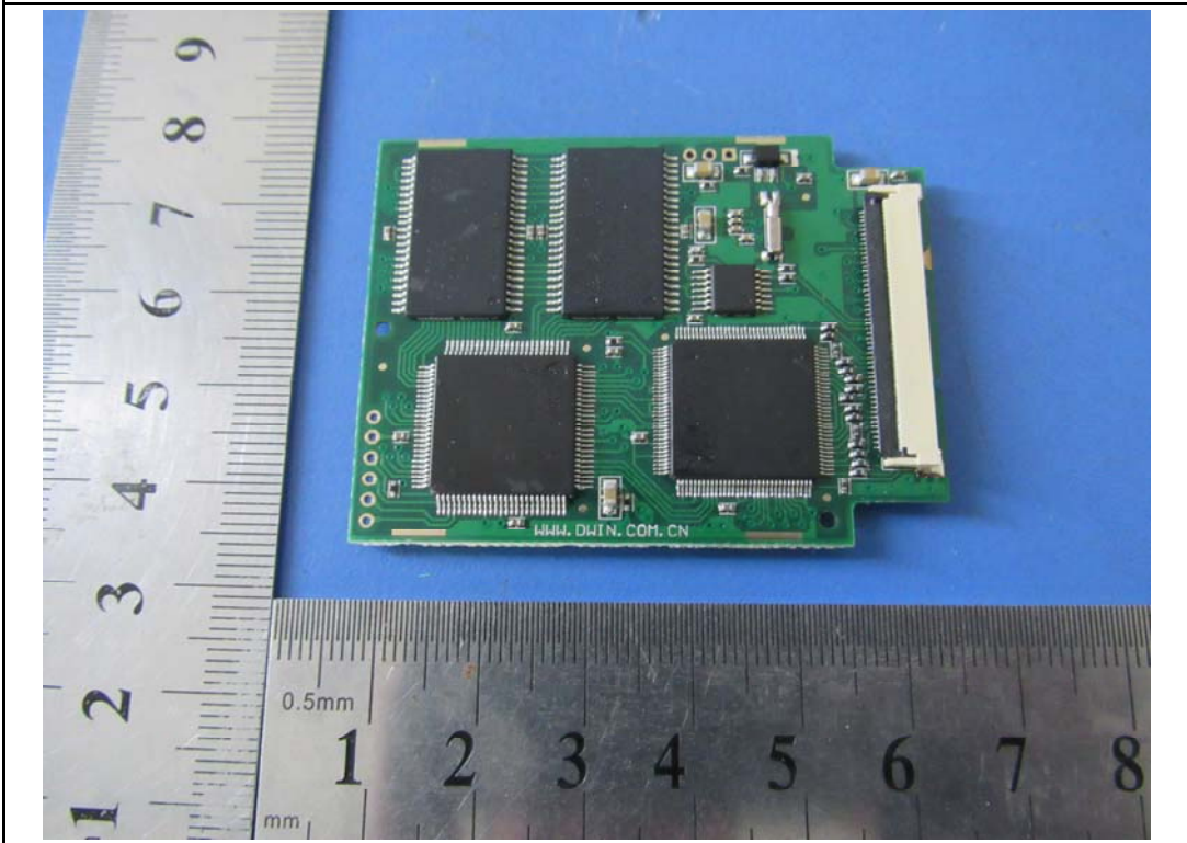
EUT - PCBA 3 Shielding Off Front View
