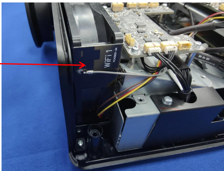
WIFI 1 Antenna
