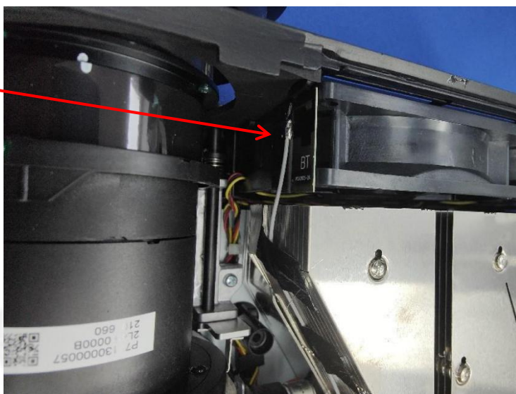
BT Antenna
