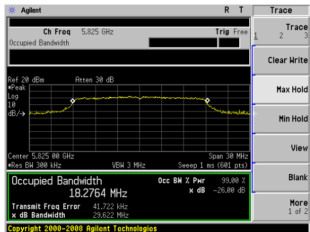
(802.11ac20) -26dB&amp;99% Bandwidth plot on channel 165
