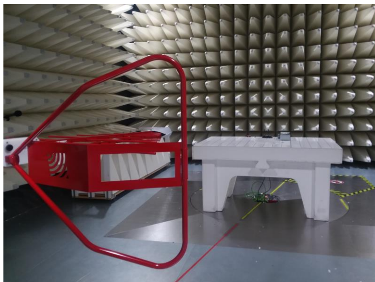
Figure D4. Radiated Emission Setup – Low Range
