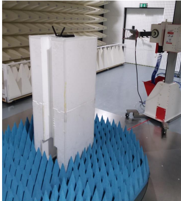
Figure D5. Radiated Emission Setup – High Range
