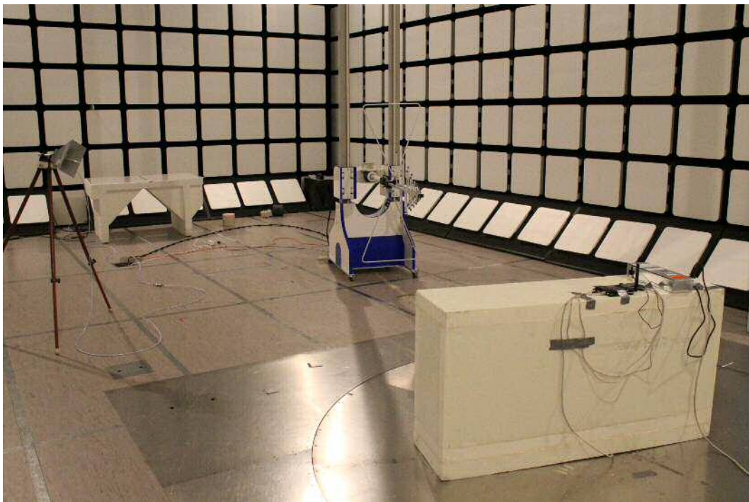
Photograph 2. Spurious emissions setup (<1 GHz)
