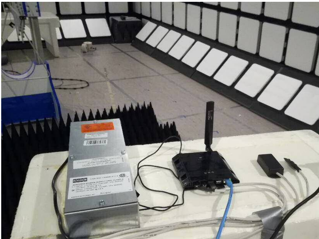
Photograph 5. Out of Band Emissions for Cellular equipment setup
