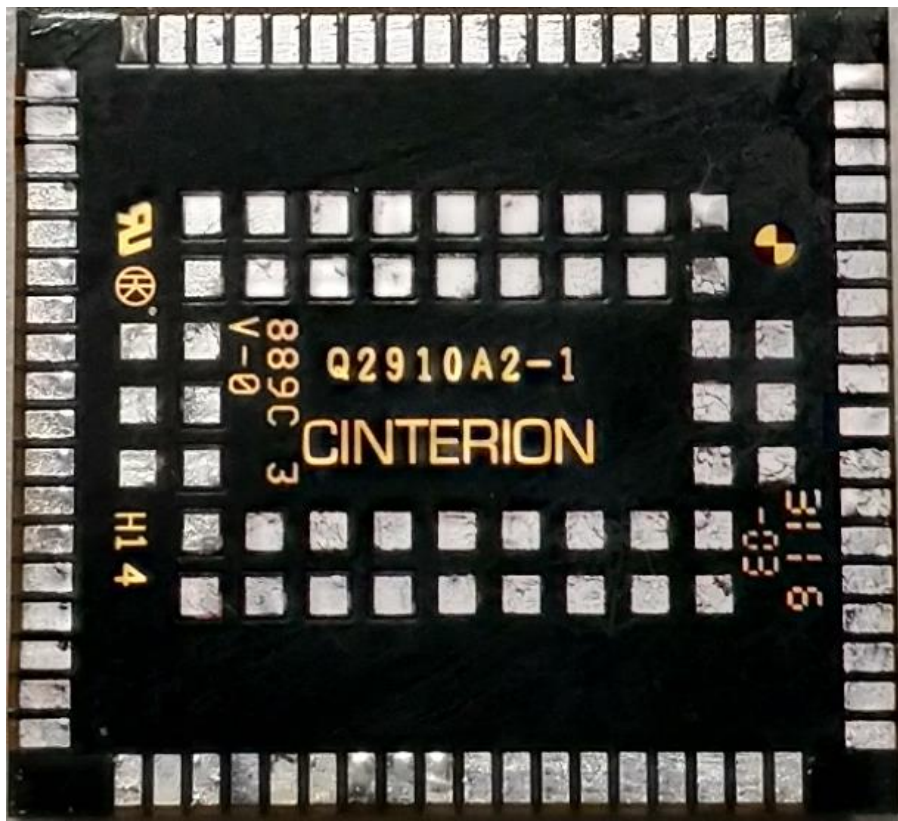
Bottom view
