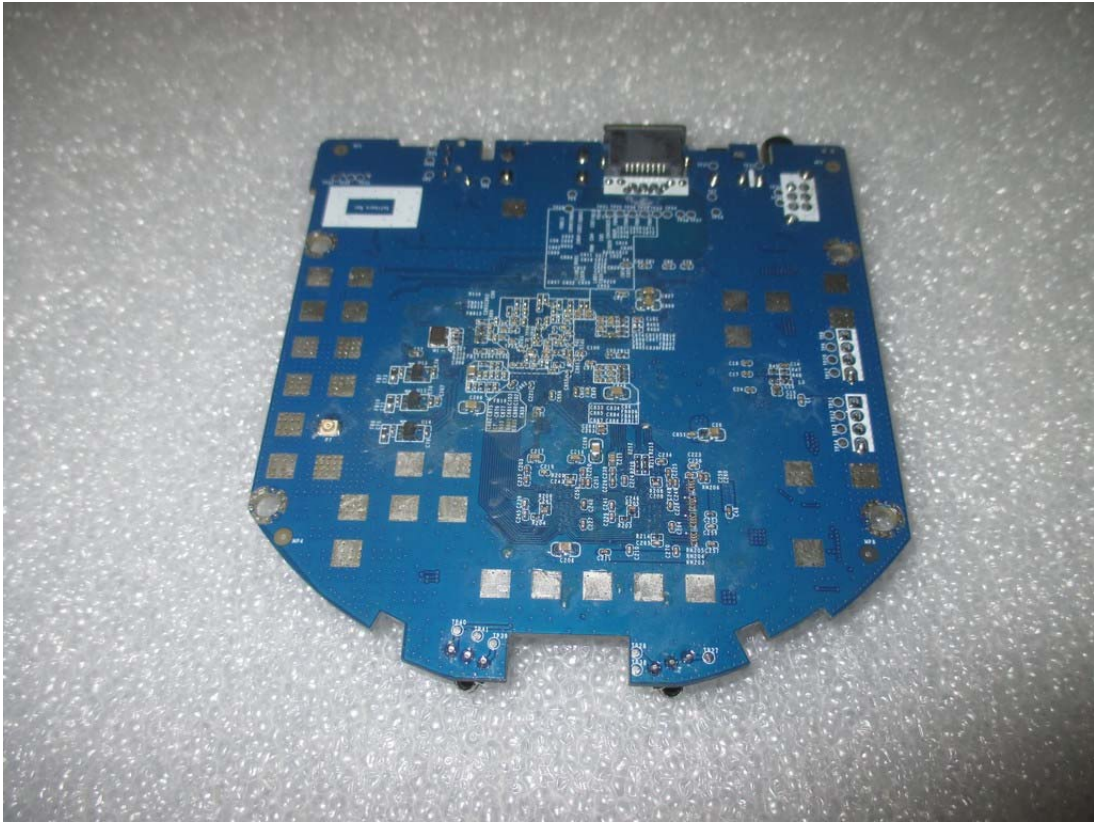
Fig. 9 PCB Rear View
