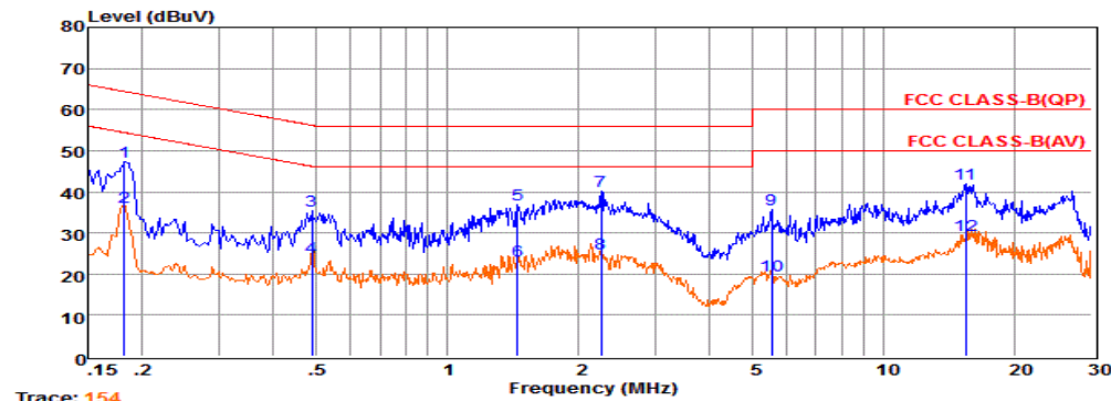
Trace: 154 Pol: NEUTRAL
