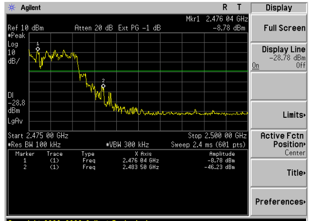
BDR mode ( \pi/4 -DQPSK): Band Edge-High Channel (Hopping Mode)
