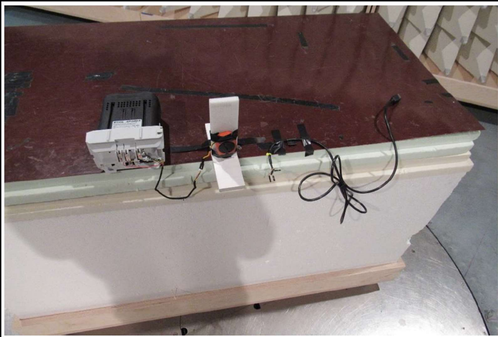
Test Setup Near View Below 1GHz
