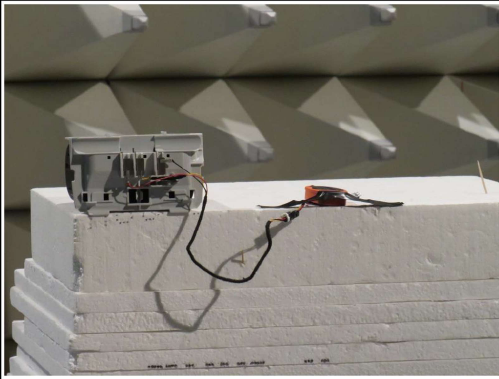
Test Setup Near View Above 1GHz - EUT horizontal
