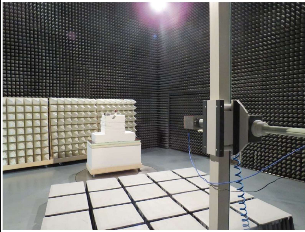
Test Setup Radiated Emissions above 18 GHz
