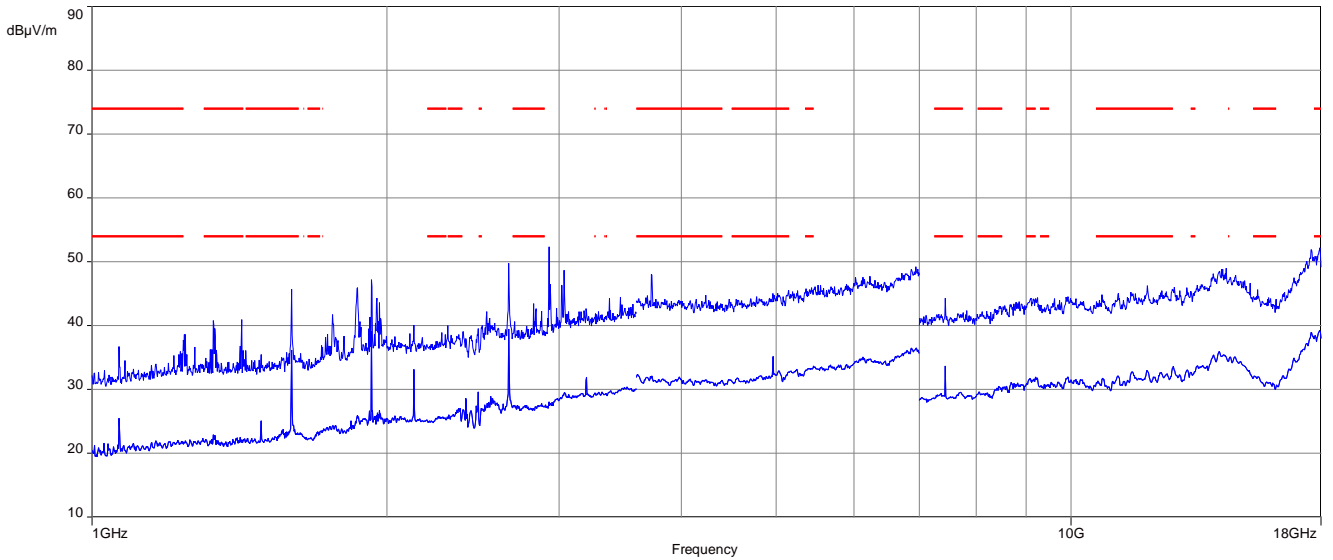
Plot 5: 1 GHz to 18 GHz, TX mode, 2480 MHz, vertical & horizontal polarization, 1 Msps, EUT position 0°
