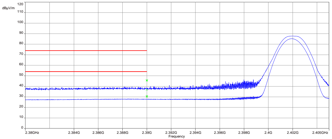
Plot 3: Lower restricted band, 1 Msps, EUT position 90°
