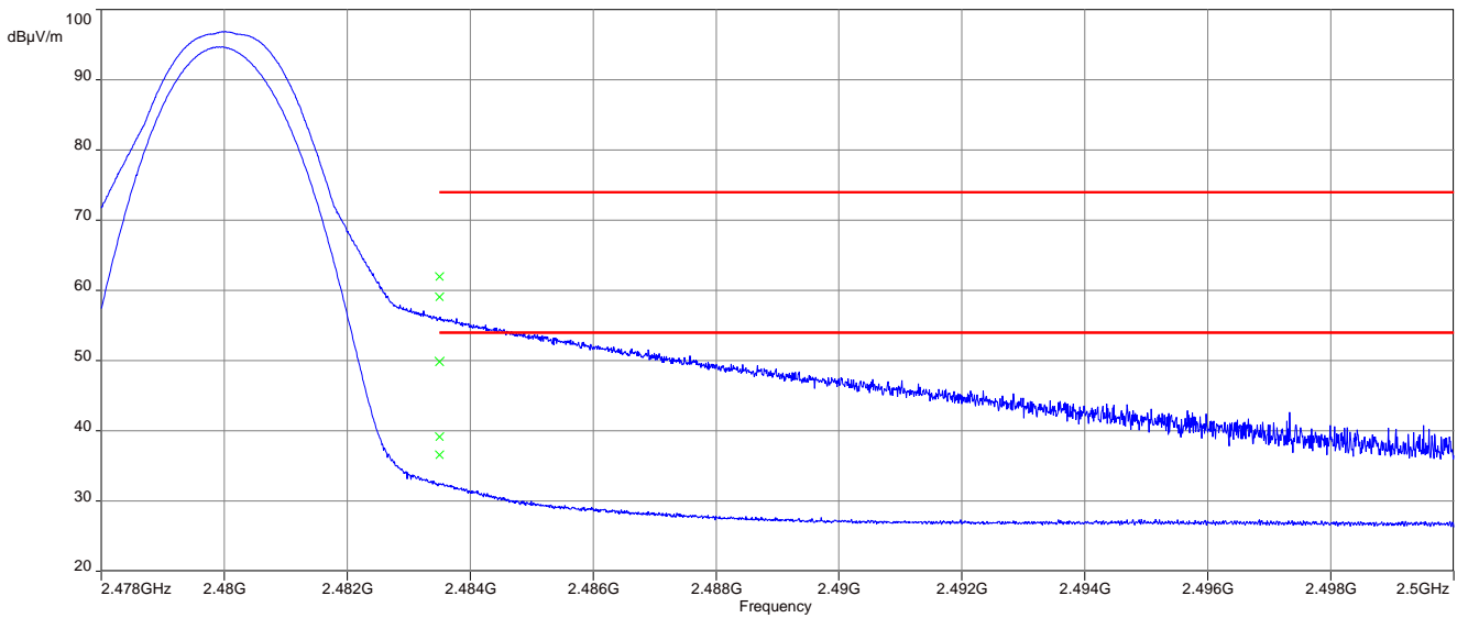
Plot 2: Upper restricted band, 1 Msps, EUT position 0°
