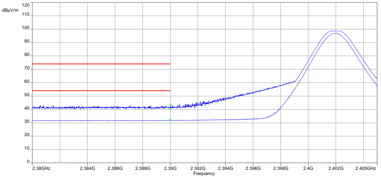
Plot 1: Lower restricted band, 1 Msps, EUT position 0°
