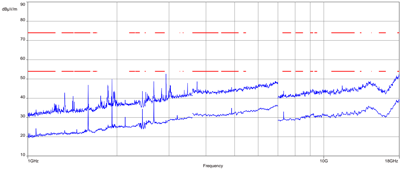
Plot 3: 1 GHz to 18 GHz, TX mode, 2440 MHz, vertical & horizontal polarization, 1 Msps, EUT position 0°
