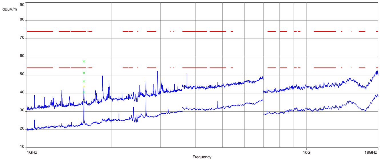
Plot 7: 1 GHz to 18 GHz, TX mode, 2402 MHz, vertical & horizontal polarization, 1 Msps, EUT position 90°
