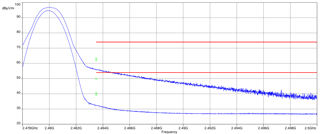
Plot 4: Upper restricted band, 1 Msps, EUT position 90°
