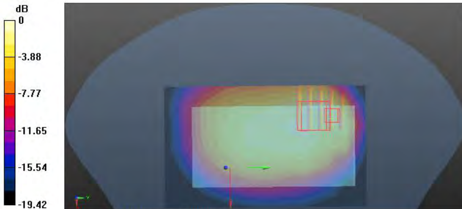
0 dB = 0.729 W/kg = -1.37 dBW/kg
