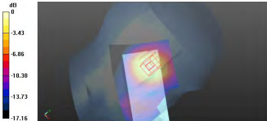
0 dB = 0.209 W/kg = -6.80 dBW/kg
