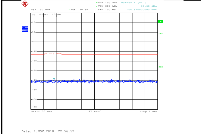
30MHz~1GHz
