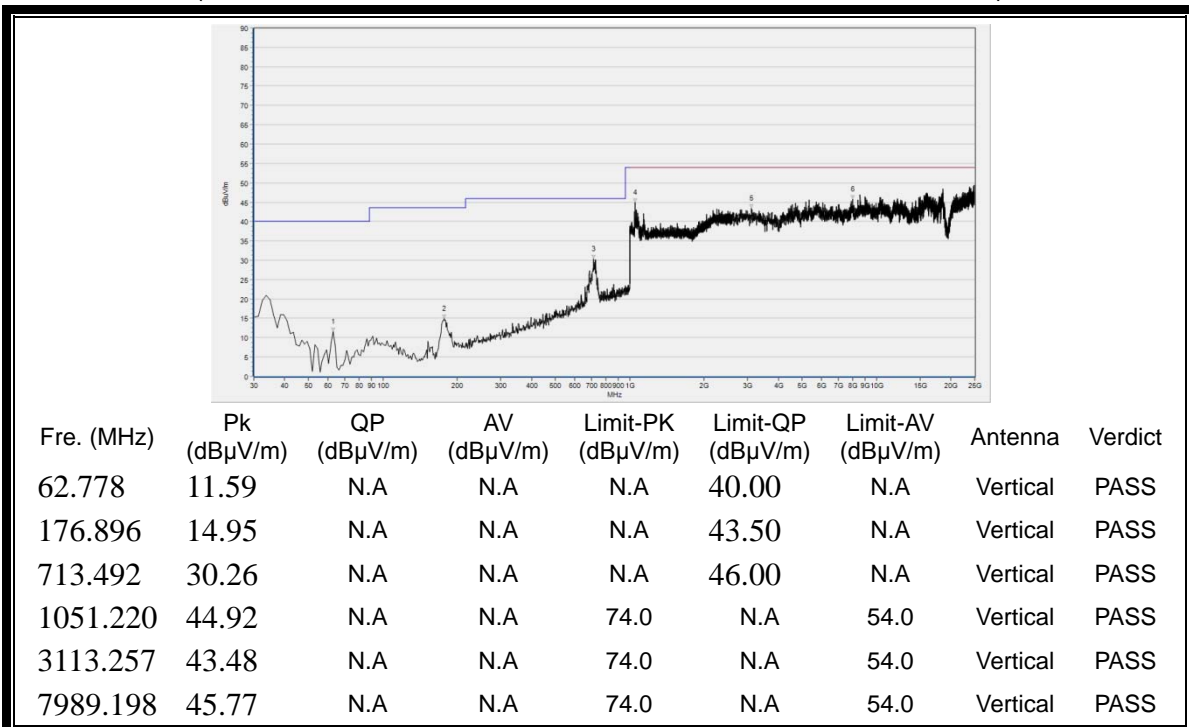
(30MHz to 25GHz, Antenna Vertical @8-DPSK, channel 39)
