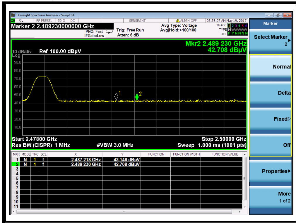
(Plot D1: Channel = 78 PEAK @ π/4-DQPSK)
