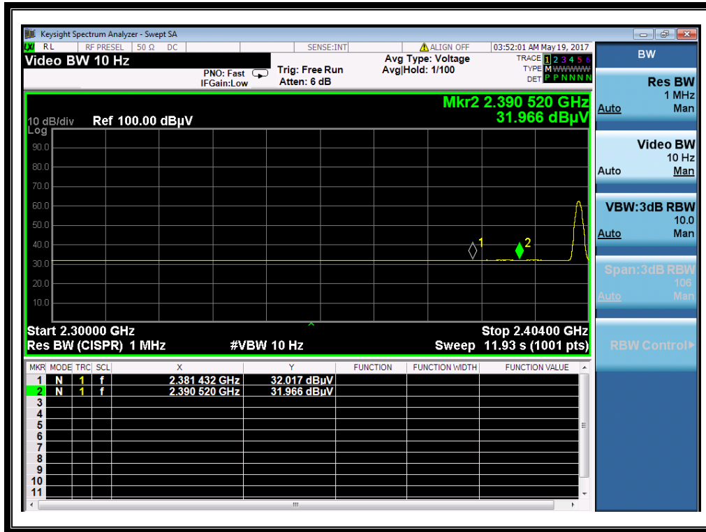
(Plot C2: Channel = 0 AVERAGE @ π/4-DQPSK)
