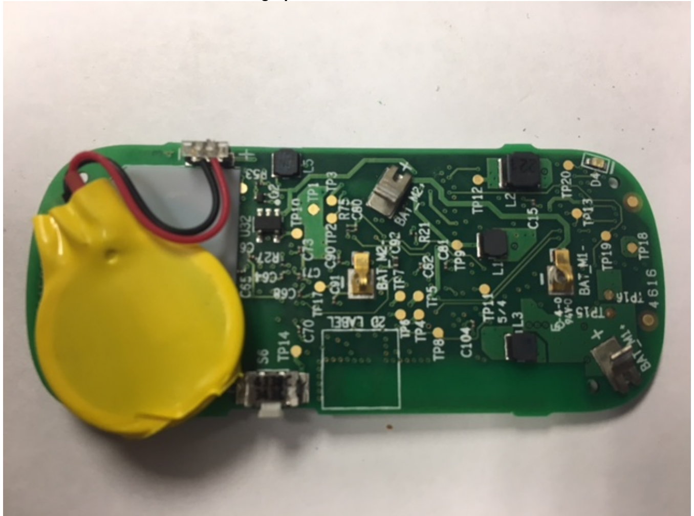
Photographs of Bottom Side of PCB
