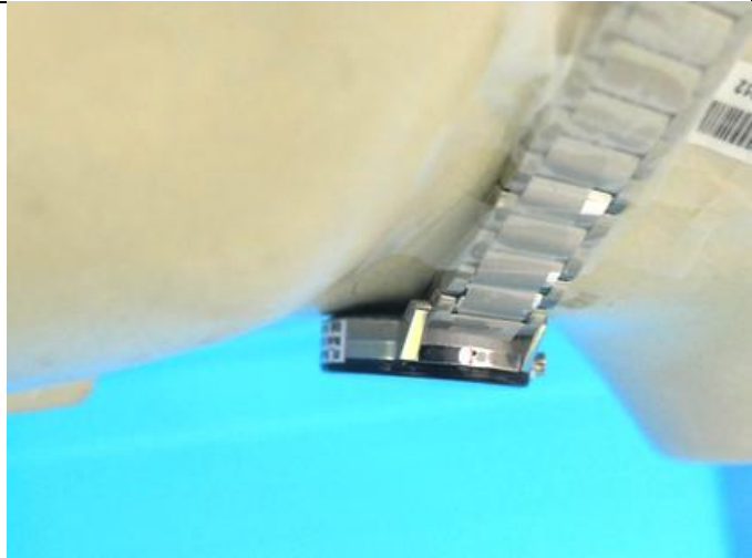
Rear Face of EUT at 0 mm_Neck Phantom_Sample 1
