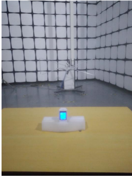
Radiated Emission test view (Frequency from 30MHz to 1GHz)
