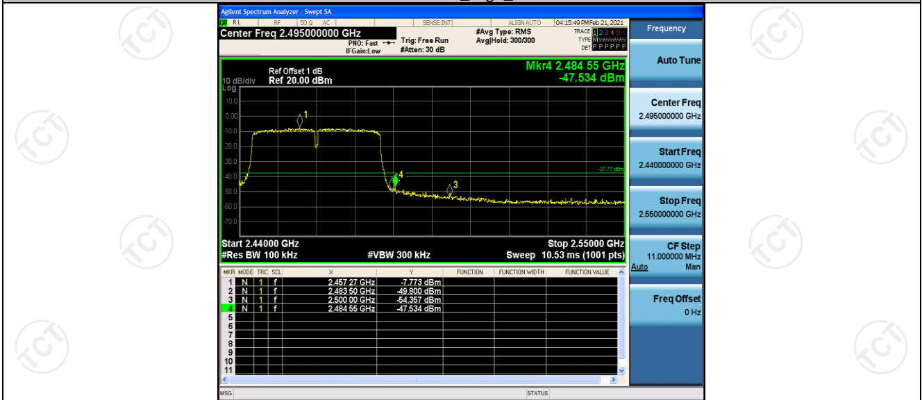
11N40SISO_High_2452
