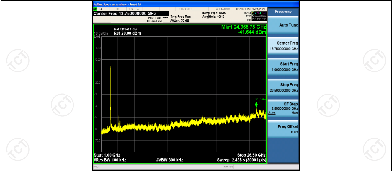
11N40SISO_2452_0~Reference
