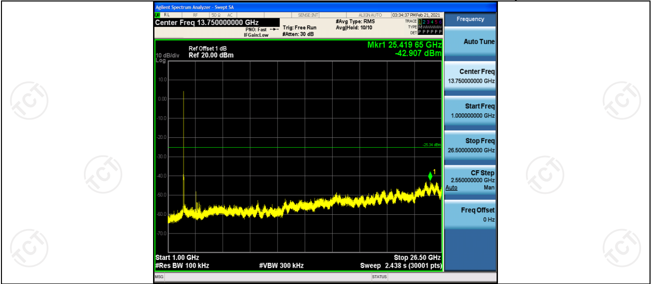
11G_2412_0~Reference
