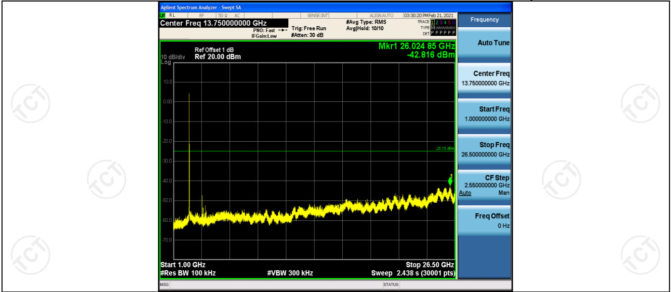
11B_2462_0-Reference
