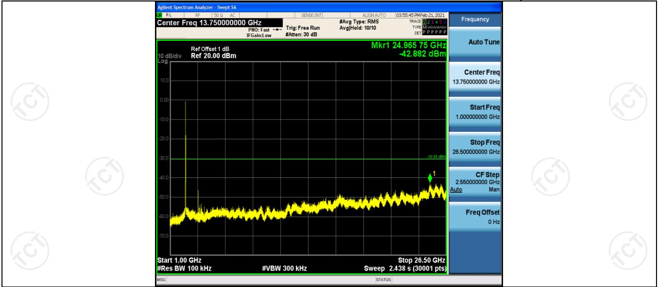
11N20SISO_2462_0~Reference
