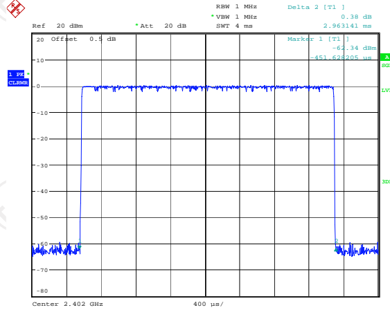
2DH5 on time (One Pulse) Plot on Channel 00
