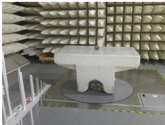
Photograph 8.2.1 Setup for final radiated emission measurements, general view
