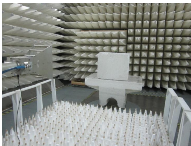
Photograph 8.1.3 Setup for final radiated emission measurements, EUT cabling
