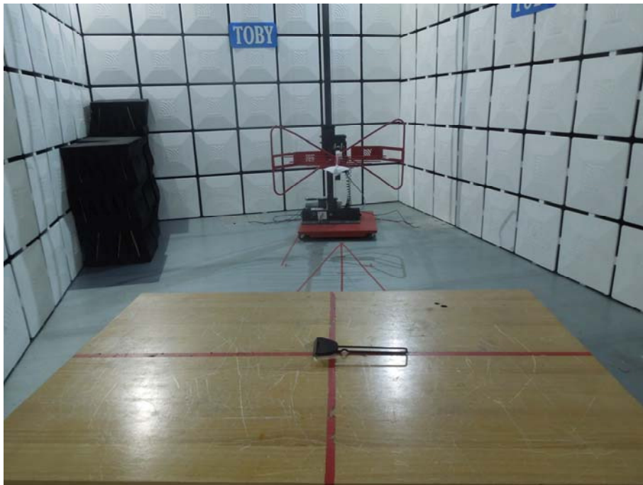
Photo of Setup for Radiated Emission (Below 1 GHz) -10 inch Ant.
