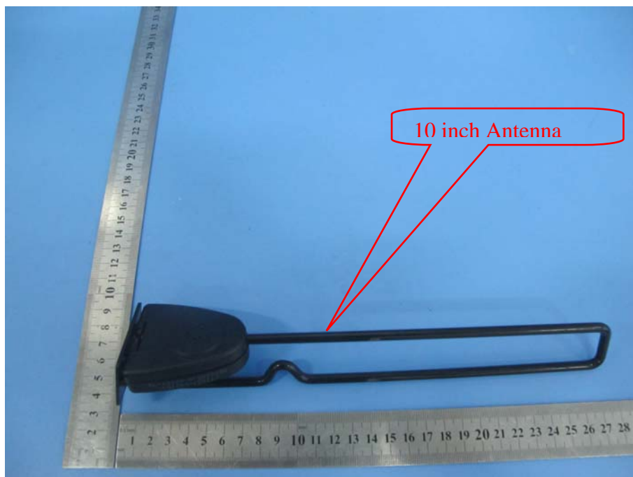
Photo 2 Appearance of EUT- Antenna(10 inch)
