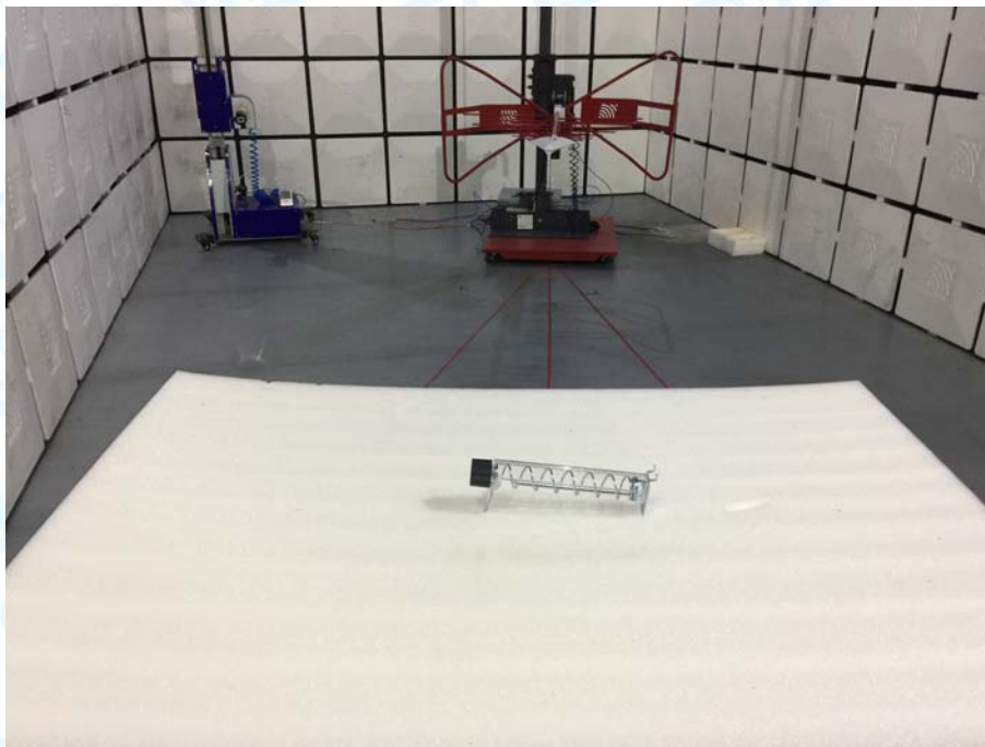
Photo of Setup for Radiated Emission (Below 1 GHz)-6 inch Antenna
