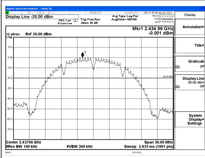
802.11b_Middle Channel
