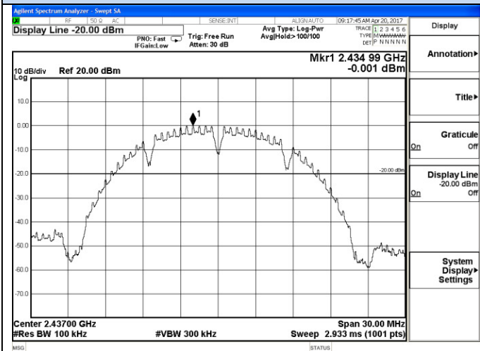
802.11b Middle channel Reference
