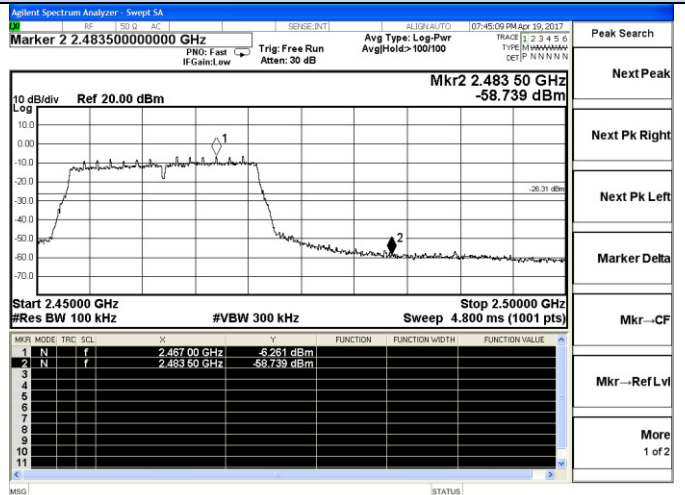
802.11n(HT40)-High channel
