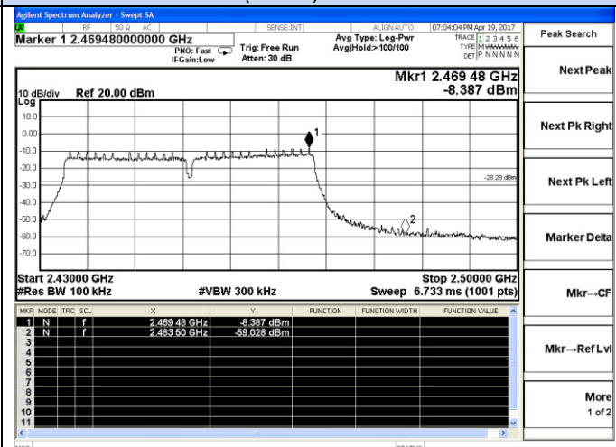
802.11n(HT20)-High channel
