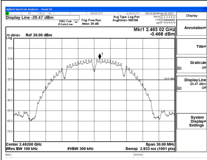
802.11b_High Channel
