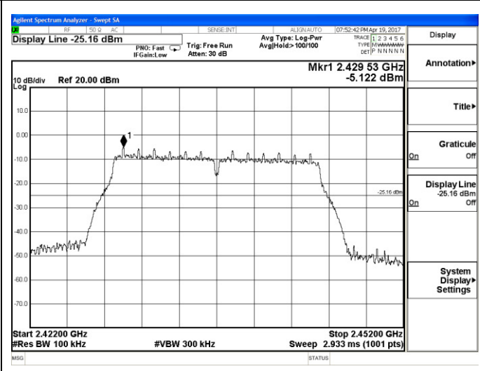
802.11g Middle channel
