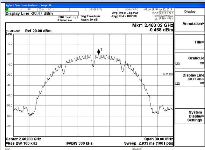
802.11b High channel Reference
