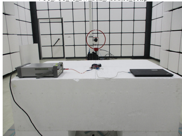
FCC_FCC_15_247_BLE_Radiated_Setup
