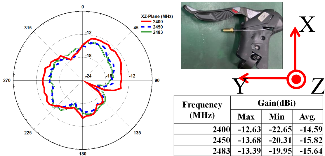
Radiation pattern_L and gain in the \Phi=0^\circ with housing
