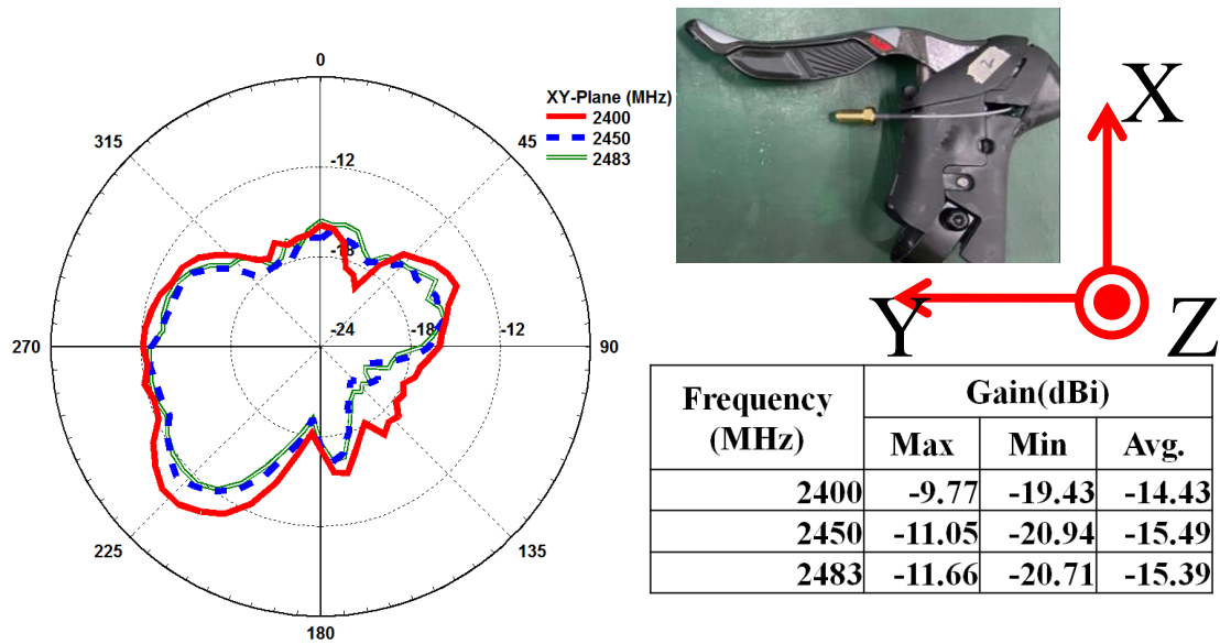
Radiation pattern_L and gain in the \theta=90^\circ with housing
