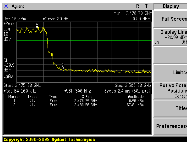
BDR mode (8DPSK): Band Edge-High Channel (Hopping Mode)
