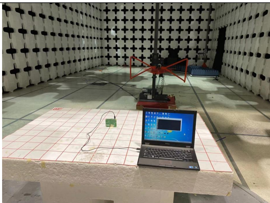
Radiated Emission Test 30MHz-1GHz Front View
