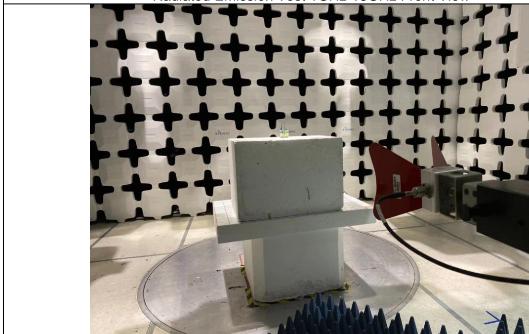
Radiated Emission Test 1GHz-18GHz Rear View
