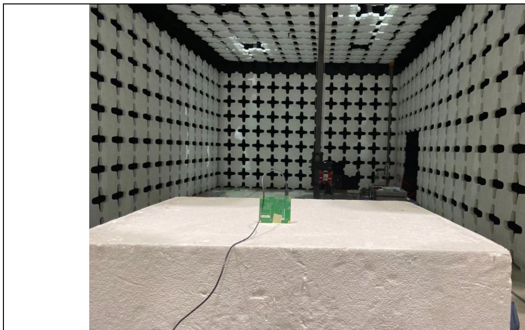
Radiated Emission Test 1GHz-18GHz Front View
