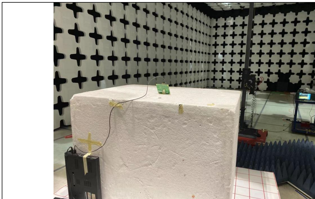
Radiated Emission Test 18GHz-40GHz Front View
